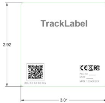
Figure 1 - TrackLabel Overall Dimensions
