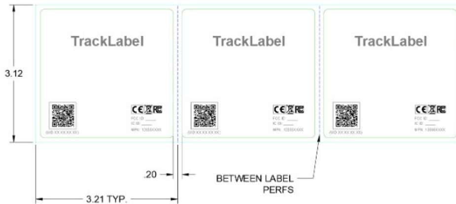
Figure 2 - TrackLabel Strip View
