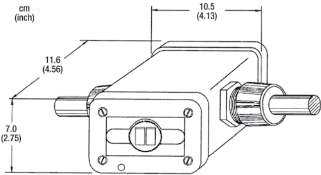
In-Line GFCI
