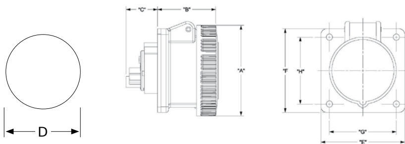
Mounting Hole
